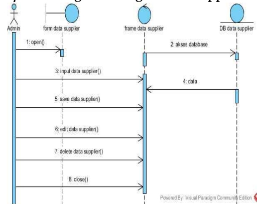
Sumber : Hasil Penelitian (2018) Gambar 9. Sequence Diagram Mengisi Data Supplier
