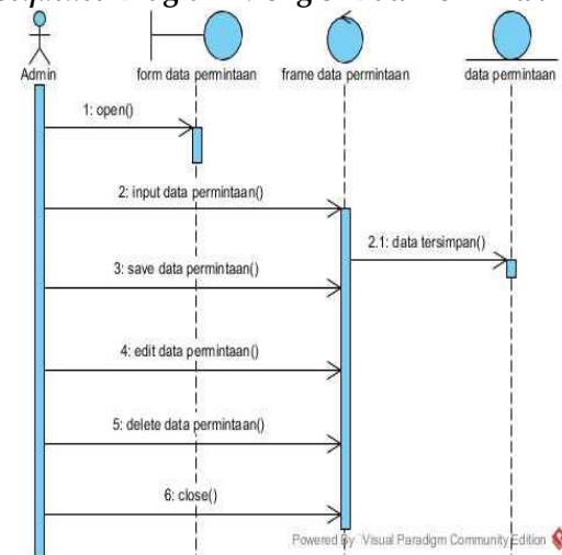
Sumber : Hasil Penelitian (2018) Gambar 10. Sequence Diagram Mengisi Data Permintaan
