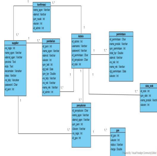
Gambar 15. Class Diagram
