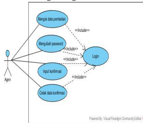
Sumber : Hasil Penelitian (2018) Gambar 2. Use Case Diagram Agen
