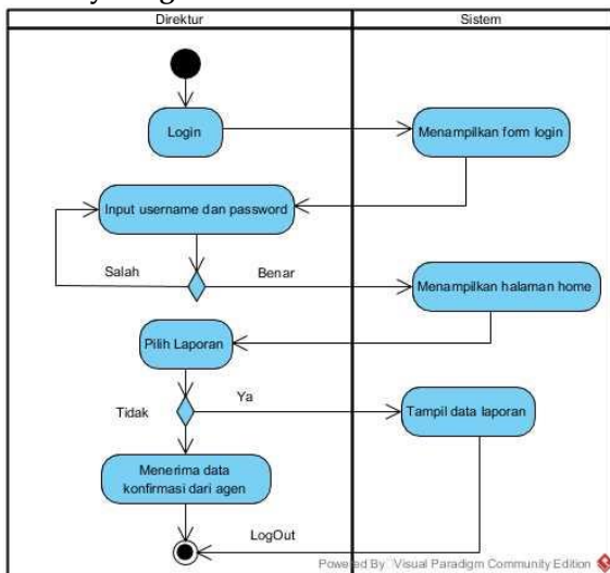
Sumber : Hasil Penelitian (2018) Gambar 6. Activity Diagram Direktur
