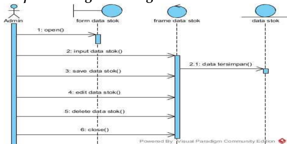
Sumber : Hasil Penelitian (2018) Gambar 7. Sequence Diagram Mengisi Data Stok
