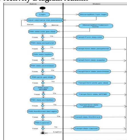
Sumber : Hasil Penelitian (2018) Gambar 4. Activity Diagram Admin
