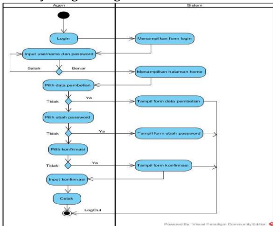
Sumber : Hasil Penelitian (2018) Gambar 5. Activity Diagram Agen
