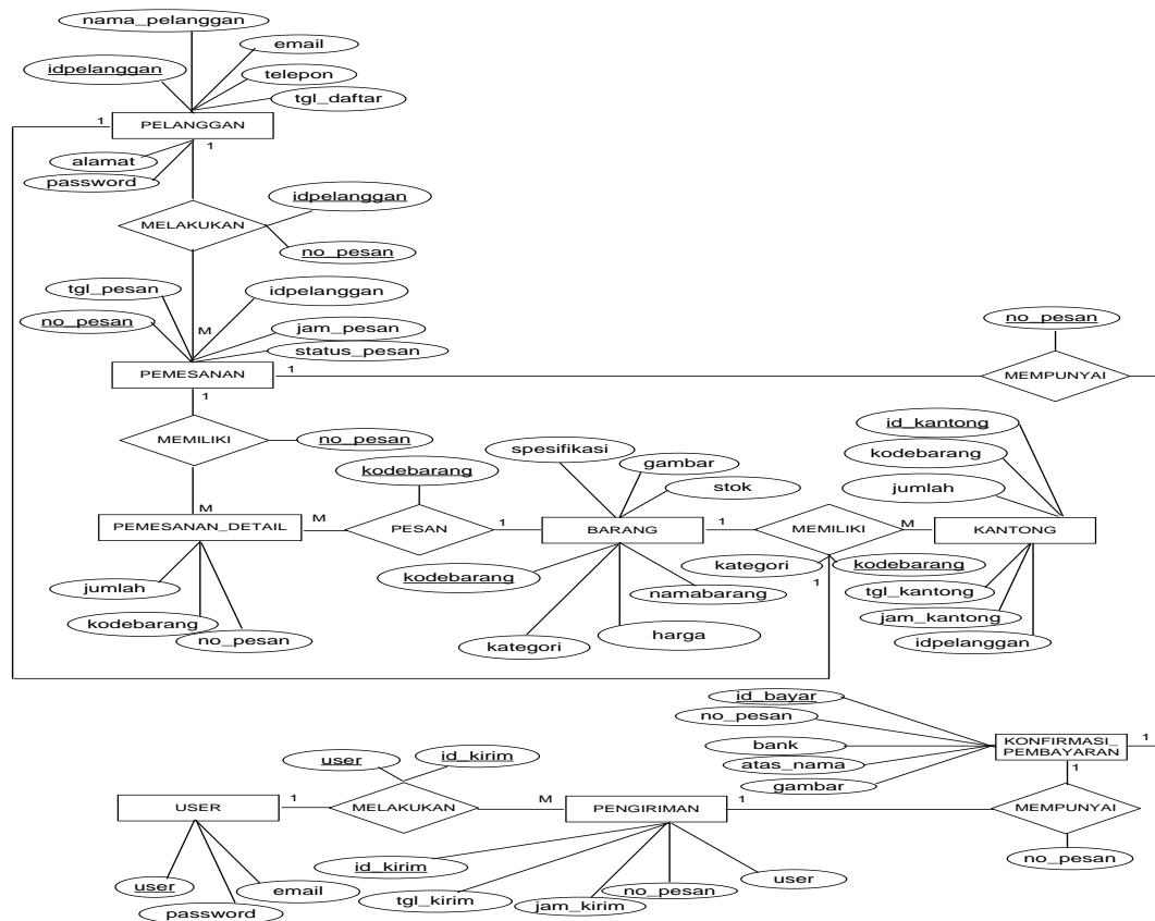
Gambar 1. Entity Relationship Diagram ( ERD) Sumber: Hasil Penelitian (2014)
